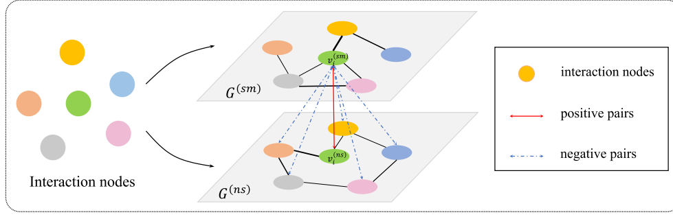
Fig. 4. The calculation process of contrastive learning loss. The solid red lines represent positive sample pairs, while the blue dashed lines represent negative sample pairs.
