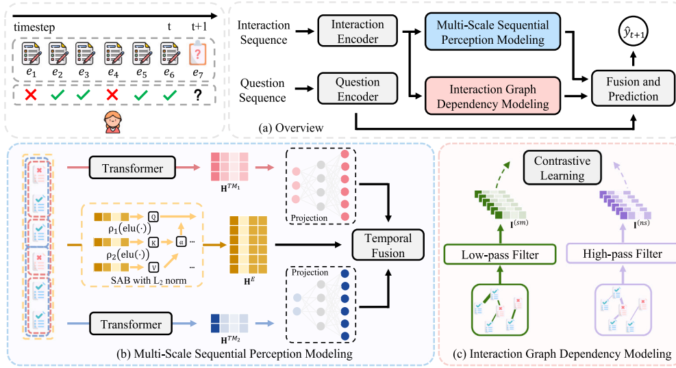
Fig. 3. The proposed MGIGKT framework. (a) is the overall workflow of the model. (b) is the Multi-Scale Sequential Perception Modeling module, dynamically modeling the student's knowledge state from a temporal perspective. (c) is the Interaction Graph Dependency Modeling module, modeling two types of interaction graphs based on similarity, and capturing the student's knowledge state from a static perspective.
