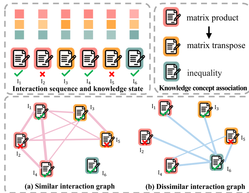
Fig. 9. Visualization of the KT process, where the upper part of the figure presents the student's historical learning records, and the lower part depicts the generated interaction graphs.
